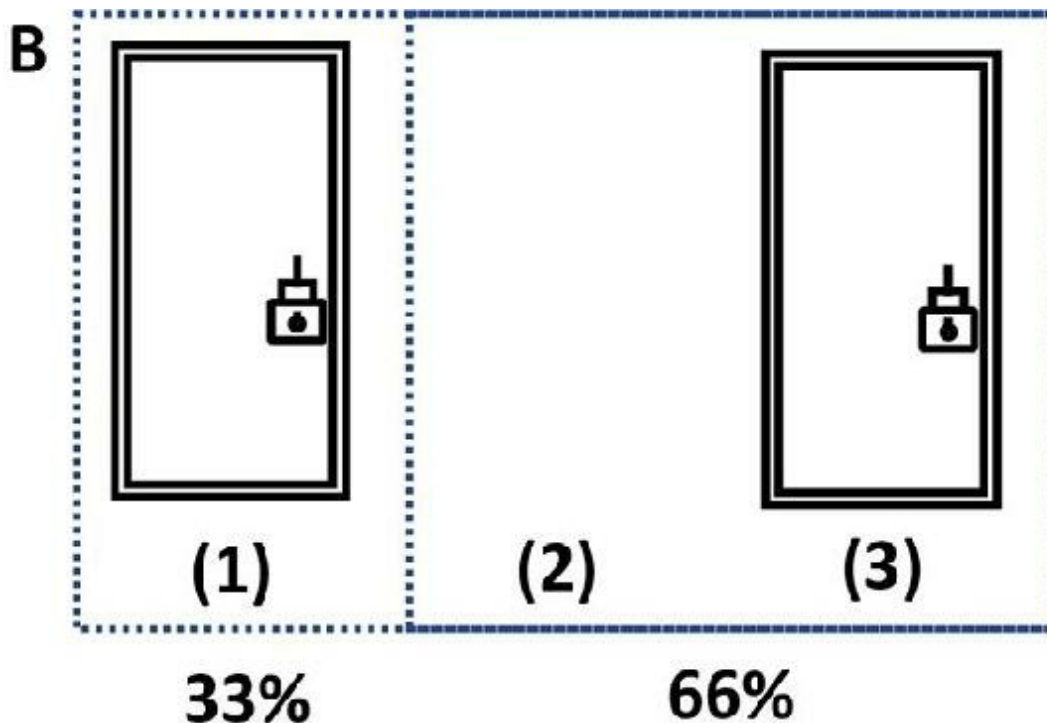
Figure 1.2: The conceptual representation of the Monty Hall problem. When a player chooses door number 1 (Figure 1.2 (A)), the probability of winning is 1/3 , or 33%. When Monty Hall then opens door number 2, the player should switch their choice, because now door number 3 offers a higher chance for winning (of 66%) (Figure 1.2 (B)).
