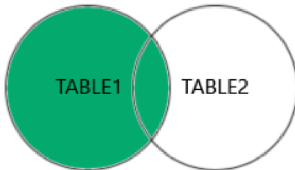
LEFT JOIN
