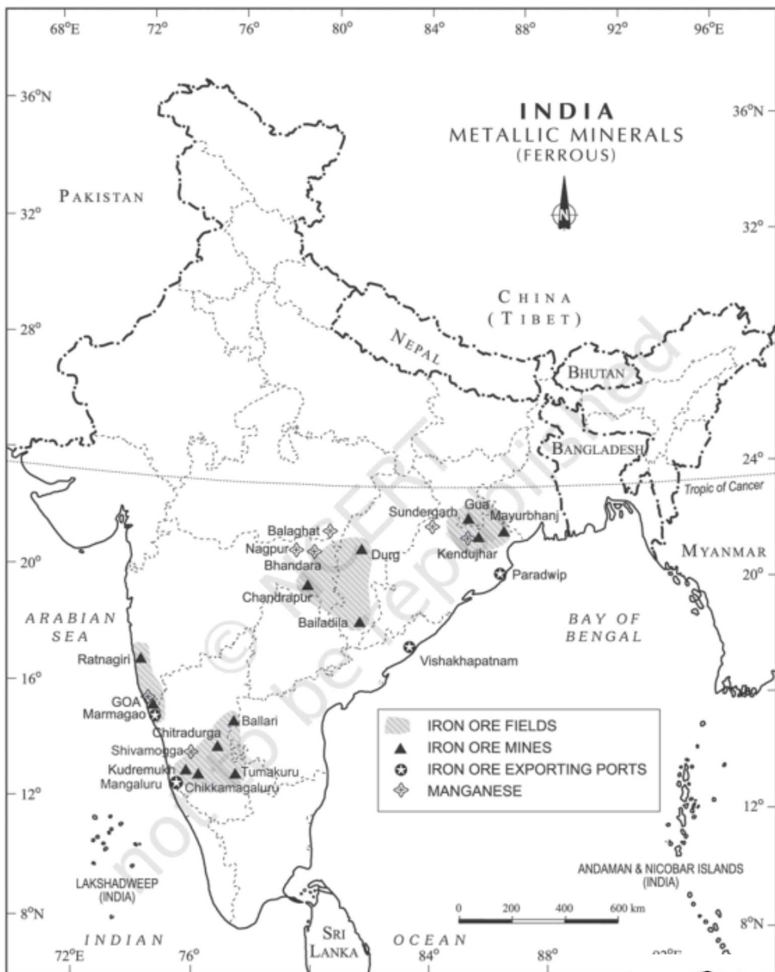
Fig. 5.2 : India - Metallic Minerals (Ferrous)
