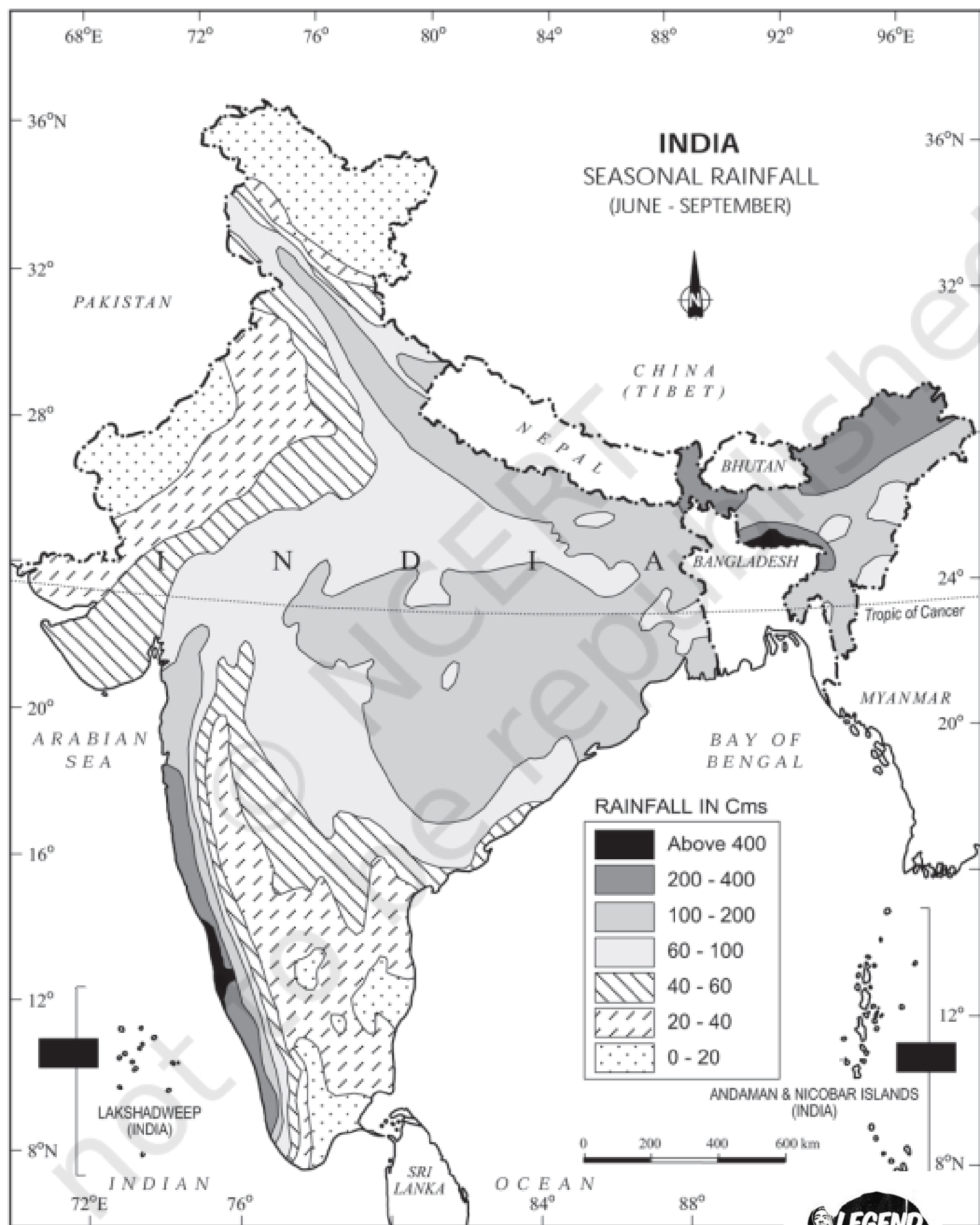
Figure 4.3 : India : Seasonal Rainfall (June-September)
