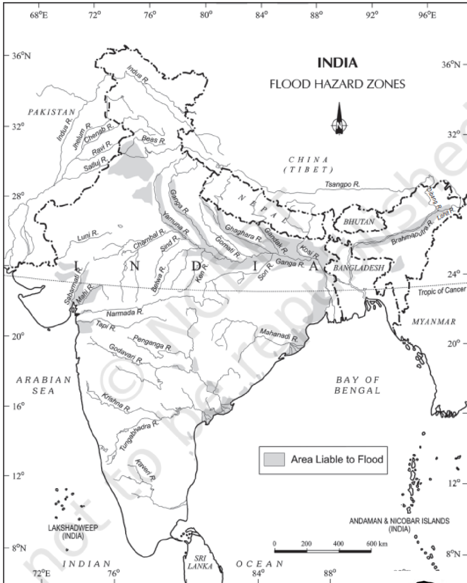
Figure 6.6 : Flood Hazard Zones
