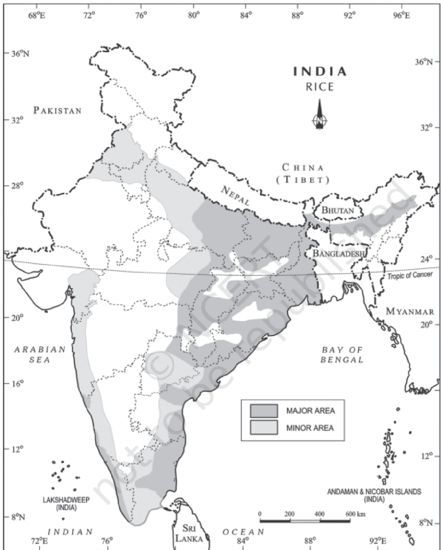
Fig. 3.3 : India - Distribution of Rice
