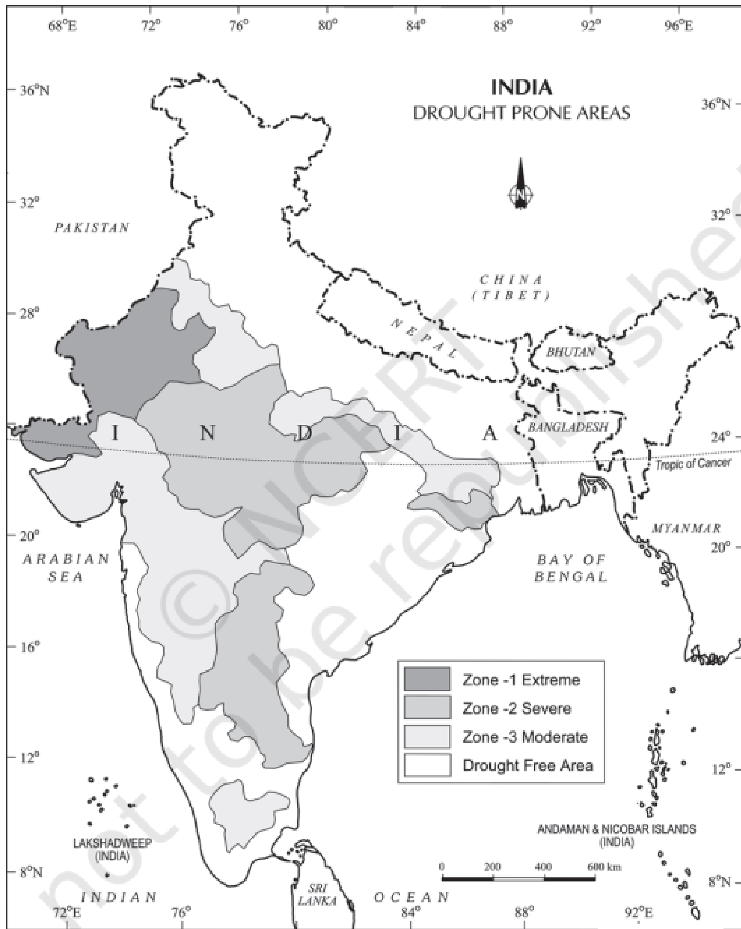
Figure 6.7 : Drought Prone Areas
