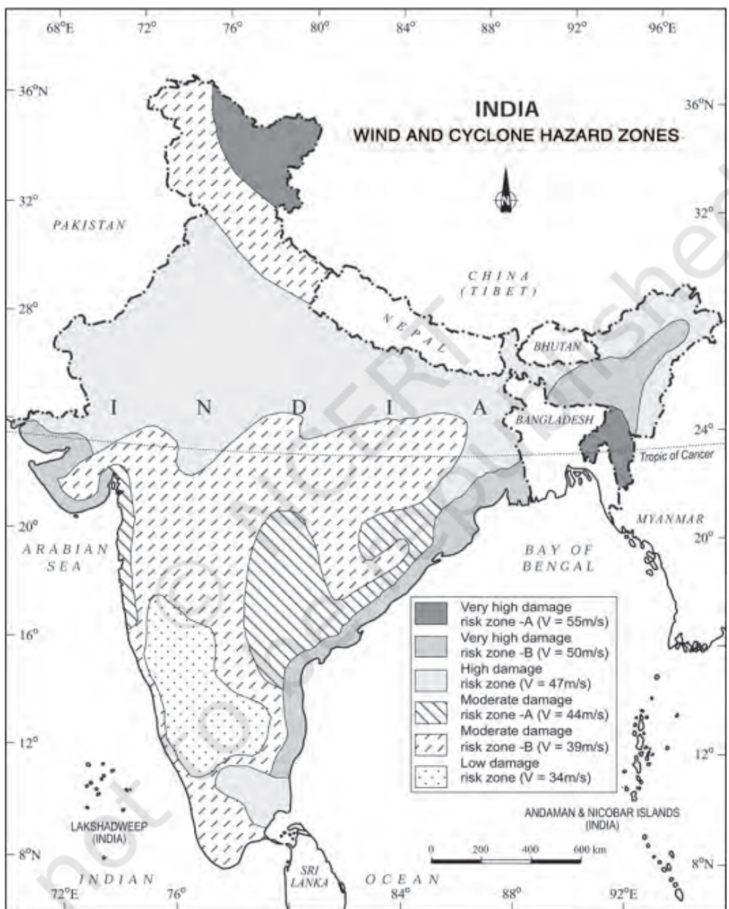
Figure 6.4 : Wind and Cyclone Hazard Zones
