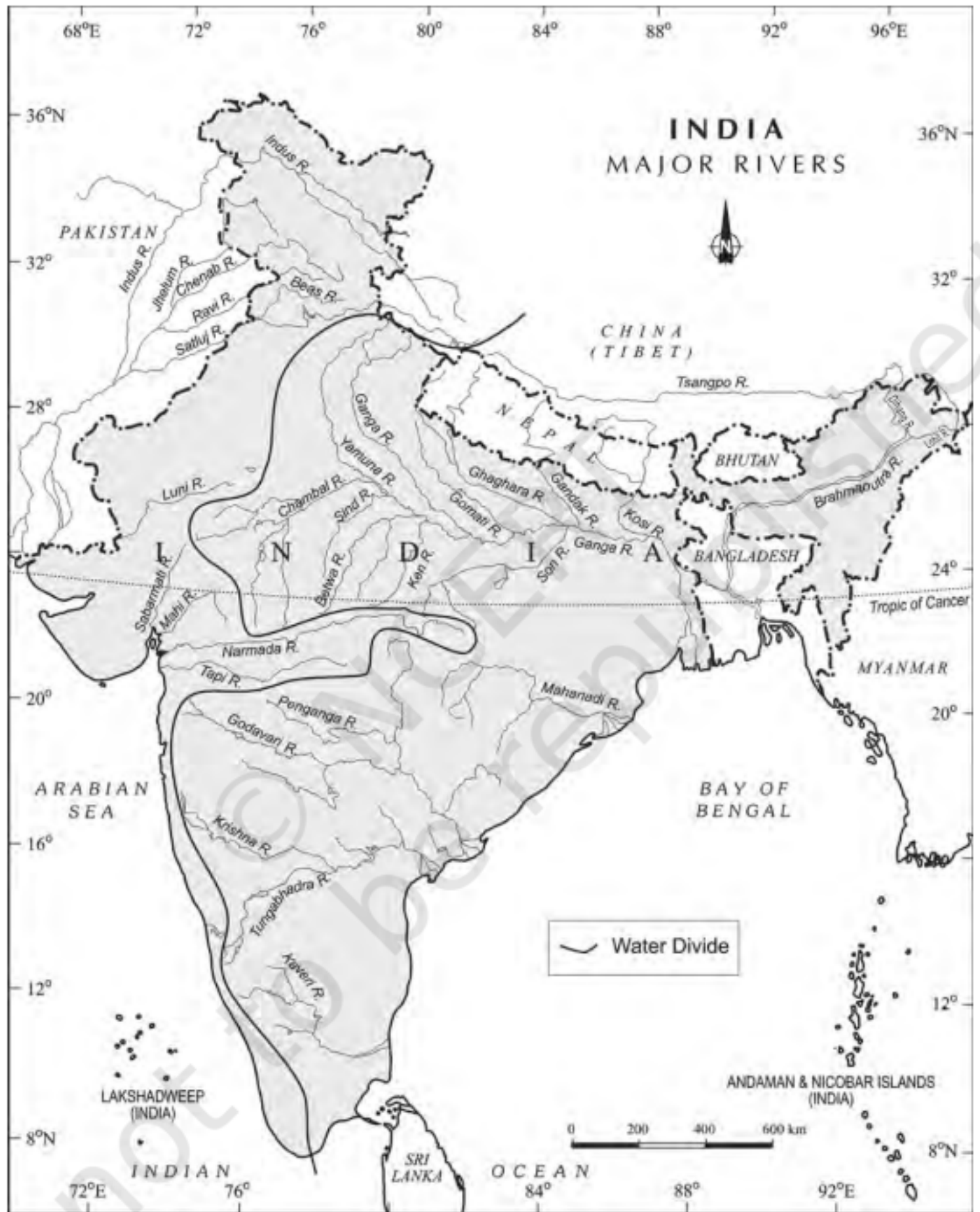
Figure 3.2 : Major Rivers of India
