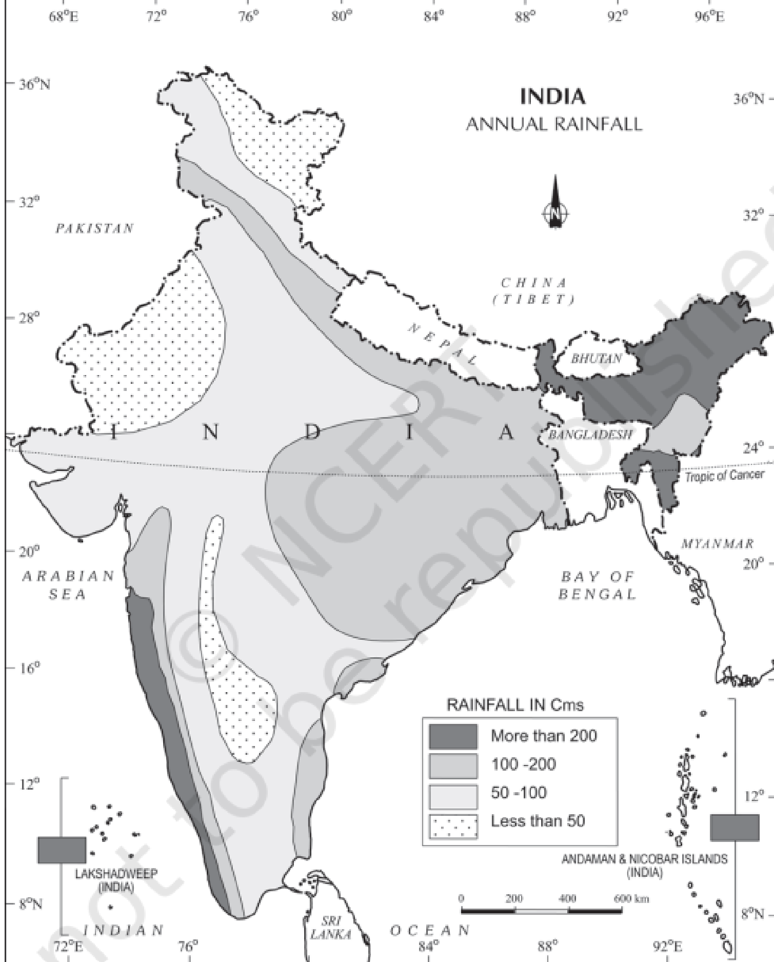
Figure 4.4 : India : Annual Rainfall
