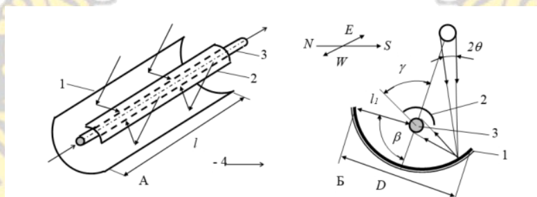
2-rasm.Parabolali konsentrator
