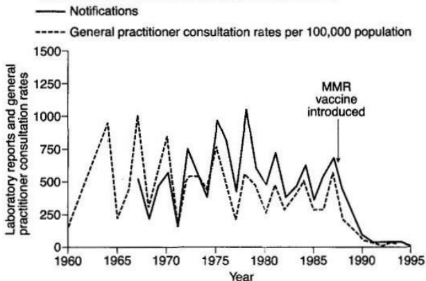
Incidence of mumps and numbers of confirmed cases reported to the Communicable Disease Surveillance Centre, 1962–95
