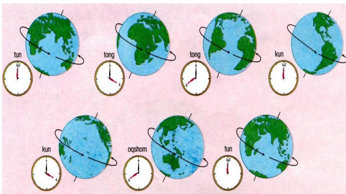
15-rasm. Yerning o'z o'qi atrofida sutkalik aylanishi
